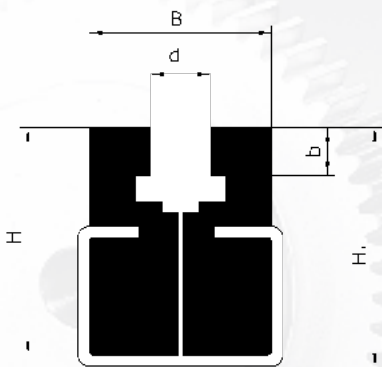
GL 1b - c ummantelt covered
